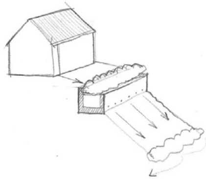
Flow through planter built into a hillside. Flows from the underdrain and overflow must be directed in accordance with City requirements.
